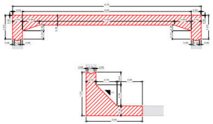
COUPES DETAILS ELEMENTS PREFA. (Scale 1/100)
